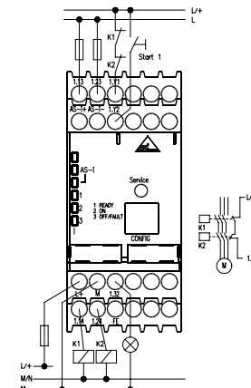
Fig. 1: Connection overview ASM1/1, ASM1E/1
