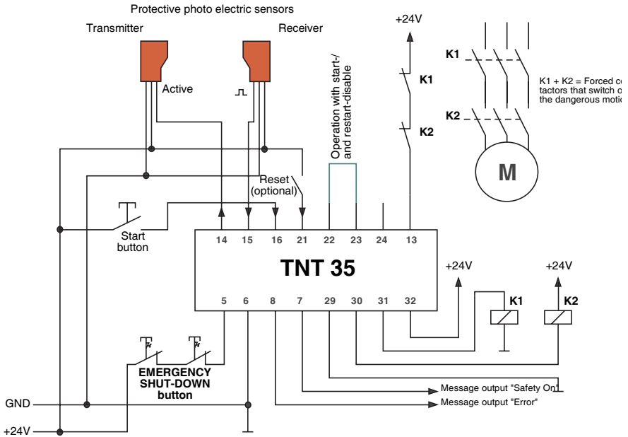
Fig. 6.5-1: Connection diagram with a protective photoelectric sensor SLS 96 and EMERGENCY SHUT-DOWN function
