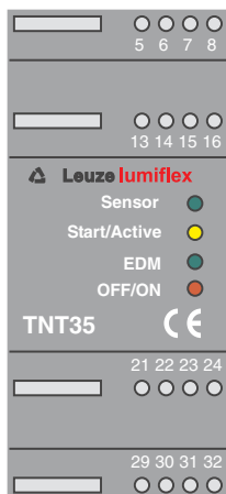
Fig. 4.1-2: Display elements TNT 35
