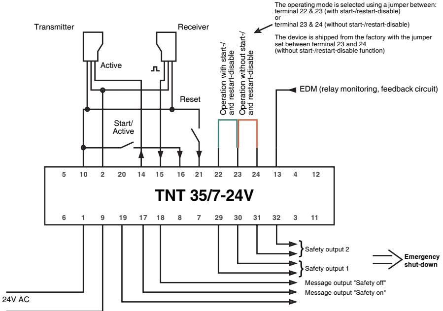
Fig. 5.1-1: Installation of the complete safety system
