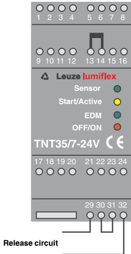
Fig. 5.2-6: Wiring safety output (one-channel release circuit)
