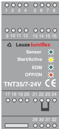
Fig. 5.5-1: Display of the TNT 35/7-24V in stand-by operation
