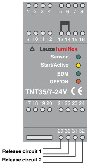
Fig. 5.2-7: Wiring safety output (two-channel release circuit)
