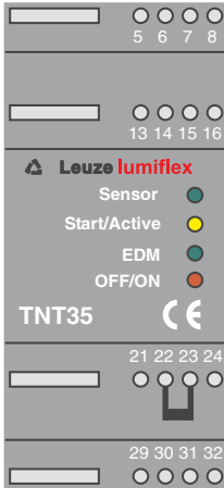
Fig. 4.2-10: Operating mode "with start- and restart-disable"
