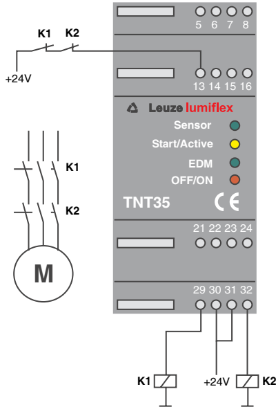
Fig. 4.2-8: Wiring of the safety output with relay monitoring
