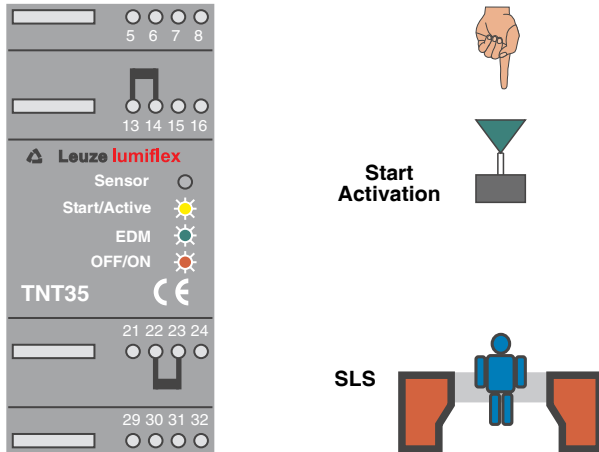
Fig. 4.4-4: Display of the TNT 35 during a safety field interruption
