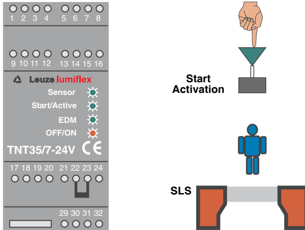
Fig. 5.5-2: Display of the TNT 35/7-24V in test operation
