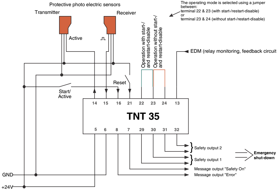
Fig. 6.2-1: Connection diagram for a pair of SLS 96s
