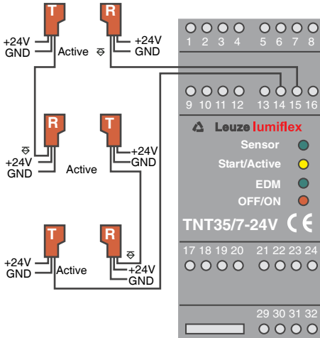
Fig. 5.2-5: Wiring of single-beam protective photoelectric sensors in series
