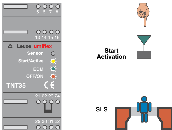
Fig. 4.5-4: Display of the TNT 35 during a safety field interruption
