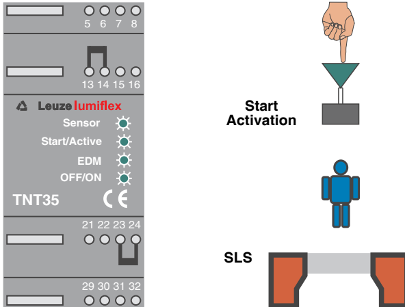
Fig. 4.3-2: Display of the TNT 35 in safety operation
