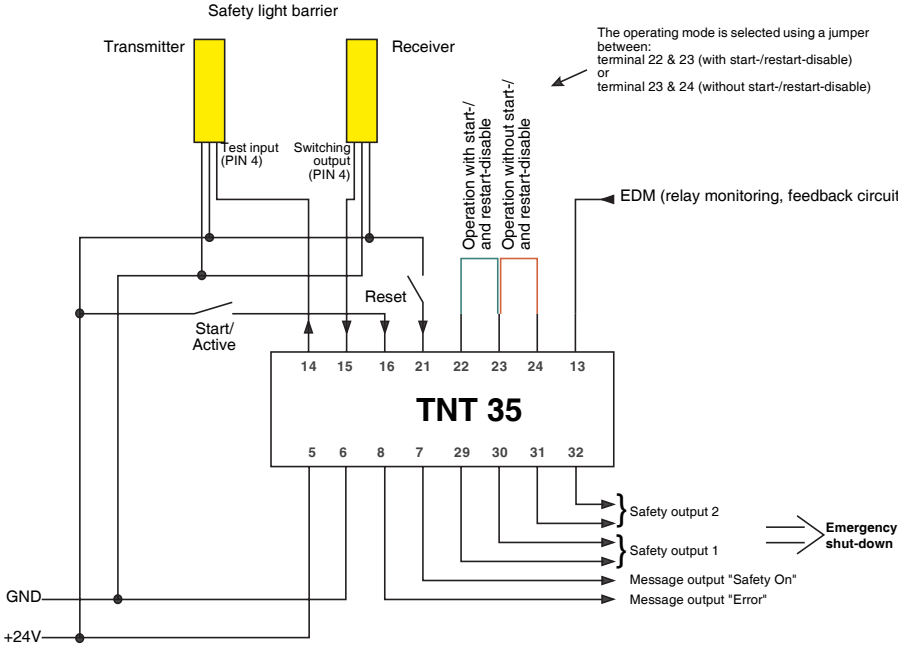
Fig. 6.3-1: Connection diagram for a pair of ECOs
