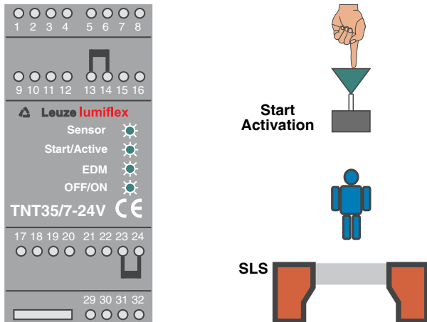
Fig. 5.3-2: Display of the TNT 35/7-24V in safety operation
