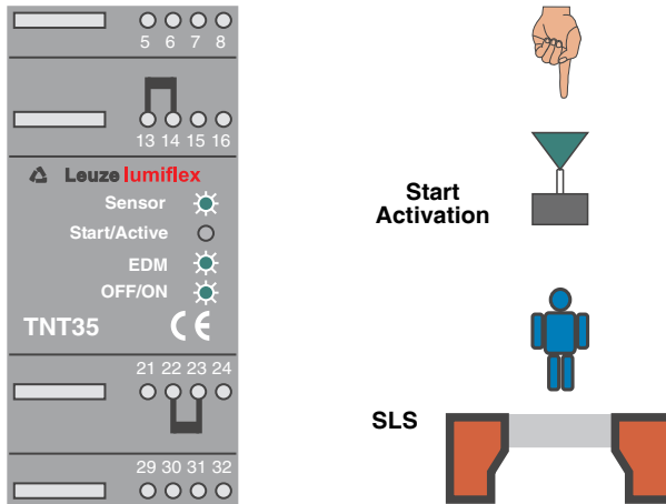
Fig. 4.4-3: Display of the TNT 35 in safety operation
