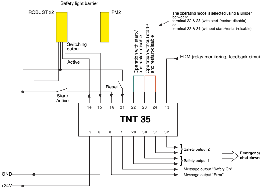
Fig. 6.4-1: Connection diagram for connecting a ROBUST 22
