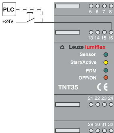
Fig. 4.2-2: Wiring of the start input "with start- and restart-disable"
