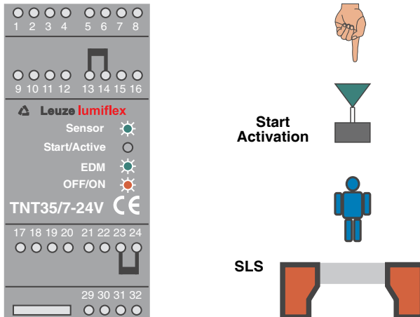
Fig. 5.3-1: Display of the TNT 35/7-24V in stand-by operation
