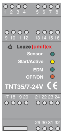
Fig. 5.1-2: Display elements TNT 35/7-24V
