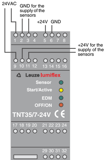
Fig. 5.2-1: Supply wiring
