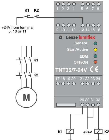
Fig. 5.2-8: Wiring of the safety output with relay monitoring
