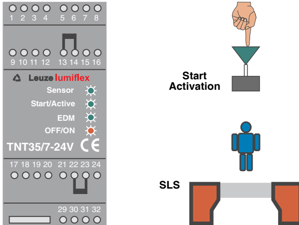
Fig. 5.4-2: Display of the TNT 35/7-24V in test operation
