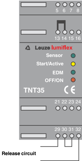
Fig. 4.2-6: Wiring safety output (one-channel release circuit)
