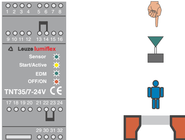
Fig. 5.4-1: Display of the TNT 35/7-24V in stand-by operation
