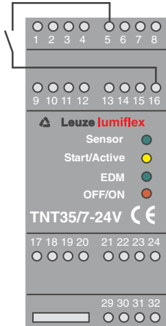
Fig. 5.2-3: Wiring of the start input "without start- and restart-disable"
