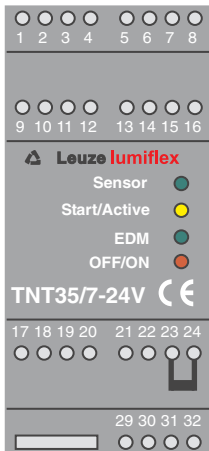
Fig. 5.2-11: Operating mode "with start- and restart-disable"
