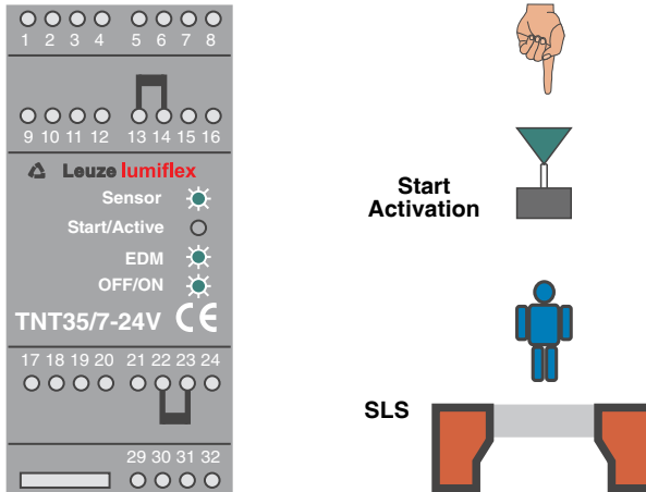
Fig. 5.4-3: Display of the TNT 35/7-24V in safety operation
