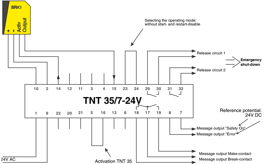
Fig. 6.6-1: Connection diagram for connecting an SRK 96
