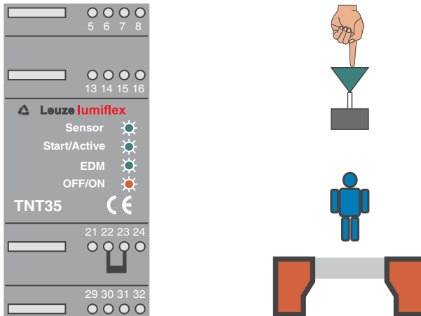
Fig. 4.5-2: Display of the TNT 35 in test operation
