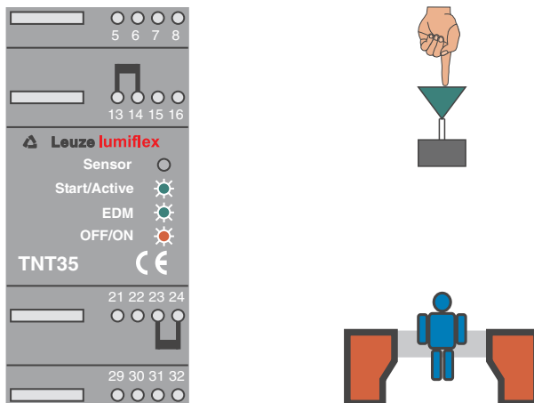
Fig. 4.3-3: Display of the TNT 35 during a safety field interruption
