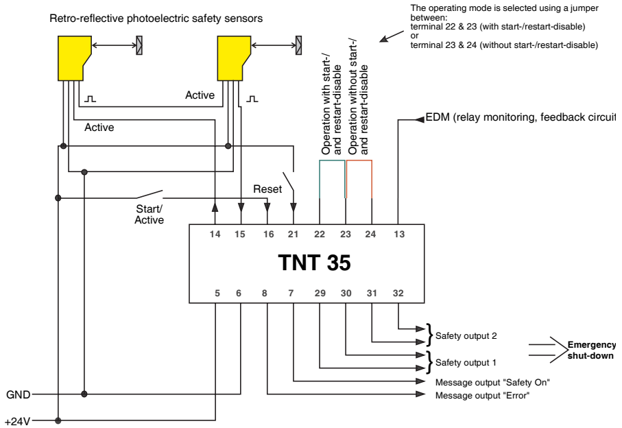
Fig. 6.1-2: Connection diagram for connecting two SRK 96s
