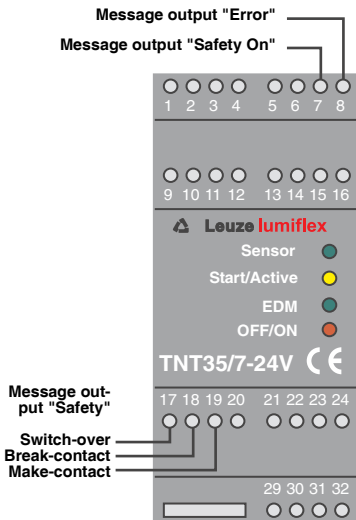
Fig. 5.2-9: Wiring of the message outputs
