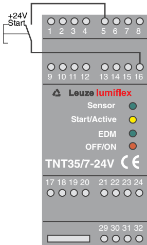
Fig. 5.2-2: Wiring of the start input "with start- and restart-disable"
