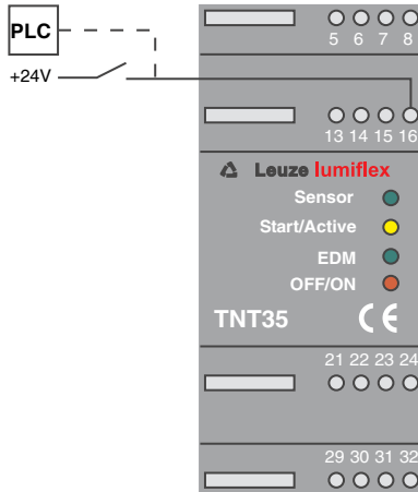
Fig. 4.2-3: Wiring of the start input "without start- and restart-disable"
