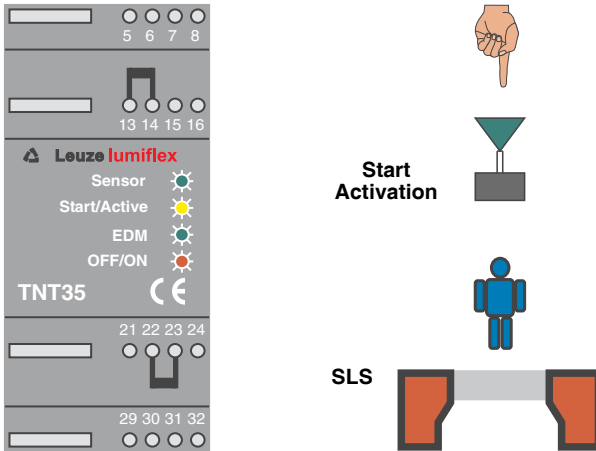
Fig. 4.4-1: Display of the TNT 35 in stand-by operation
