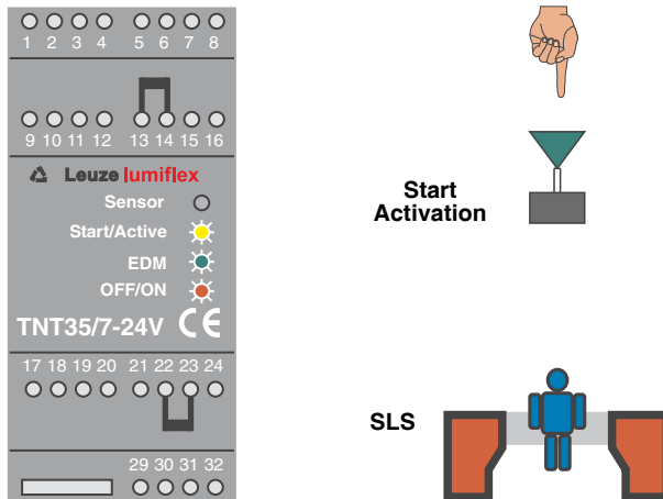
Fig. 5.4-4: Display of the TNT 35/7-24V during a safety field interruption
