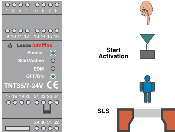
Fig. 5.5-3: Display of the TNT 35/7-24V in safety operation
