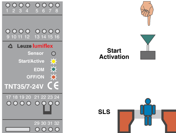
Fig. 5.5-4: Display of the TNT 35/7-24V during a safety field interruption
