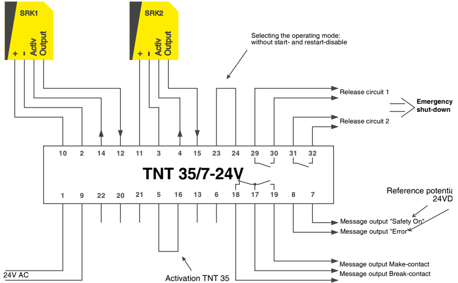
Fig. 6.7-1: Connection diagram for connecting two SRK 96s
