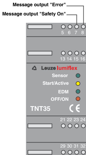
Fig. 4.2-9: Wiring of the message outputs
