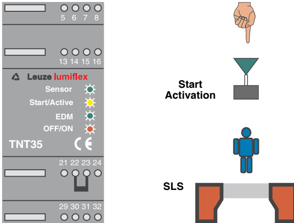
Fig. 4.5-1: Display of the TNT 35 in stand-by operation
