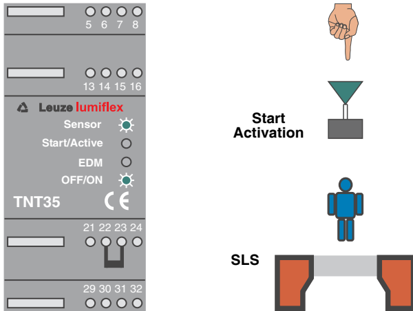
Fig. 4.5-3: Display of the TNT 35 in safety operation
