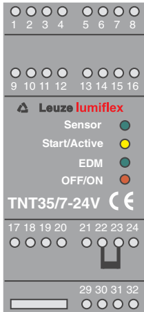
Fig. 5.2-10: Operating mode "with start- and restart-disable"
