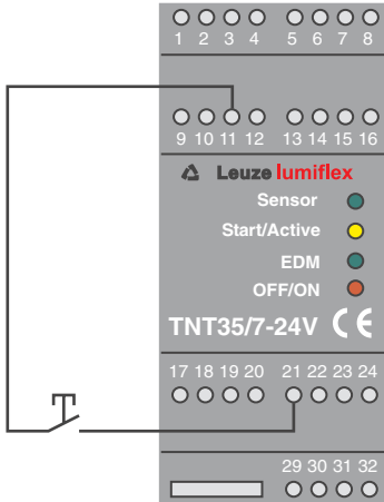
Fig. 5.6-1: Resetting from a locked state
