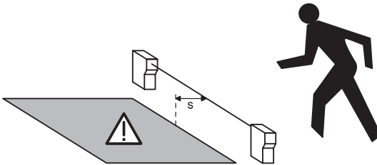
Fig. 3.1-1: Safety distance S between photoelectric sensor and hazardous area
