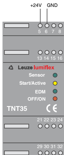
Fig. 4.2-1: Supply wiring
