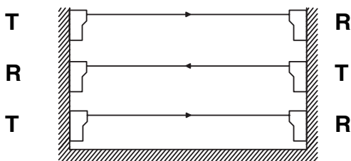
Fig. 3.1-2: Multi-axe installation
