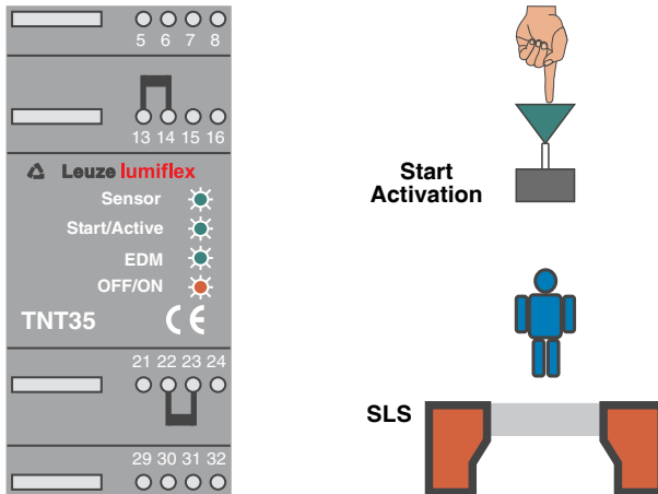
Fig. 4.4-2: Display of the TNT 35 in test operation
