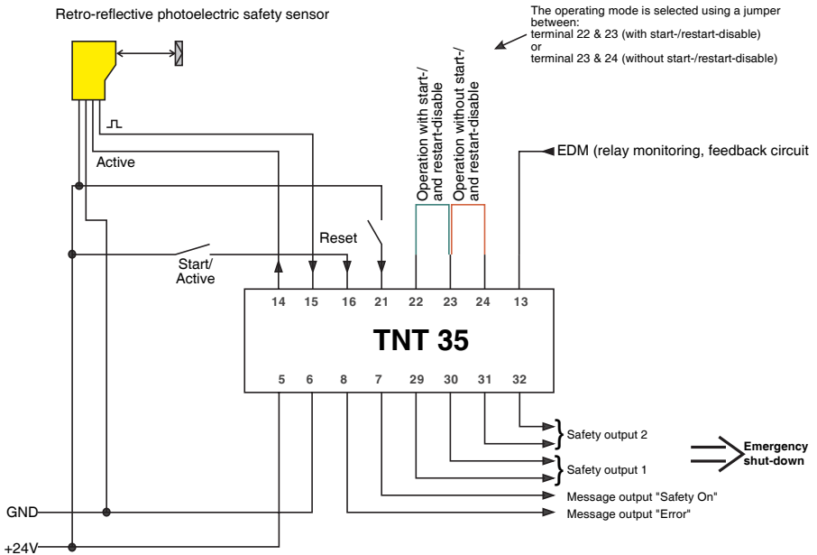
Fig. 6.1-1: Connection diagram for connecting an SRK 96
