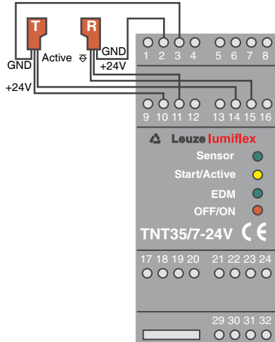
Fig. 5.2-4: Wiring of single-beam protective photoelectric sensors
