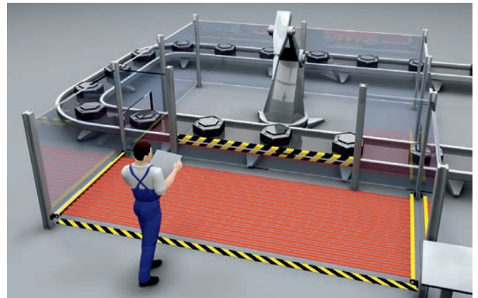
Safeguarding danger areas with horizontal installation of a light curtain with 40 mm resolution on a robot cell
